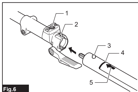
Fig. 6 ► 1. Release button 2. Arrow mark on the power unit 3. Pin 4. Position line 5. Arrow mark on the pipe
